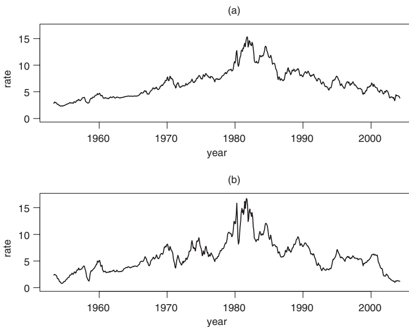
Figure 1.5. Time plots of monthly U.S. interest rates from April 1953 to March 2004: (a) the 10-year Treasury constant maturity rate and (b) the 1-year maturity rate.
