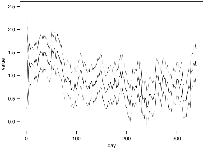
Figure 11.3. Filtered state variable \mu_{r|t} and its 95% pointwise confidence interval for the daily log realized volatility of Alcoa stock returns based on the fitted local trend state-space model.
