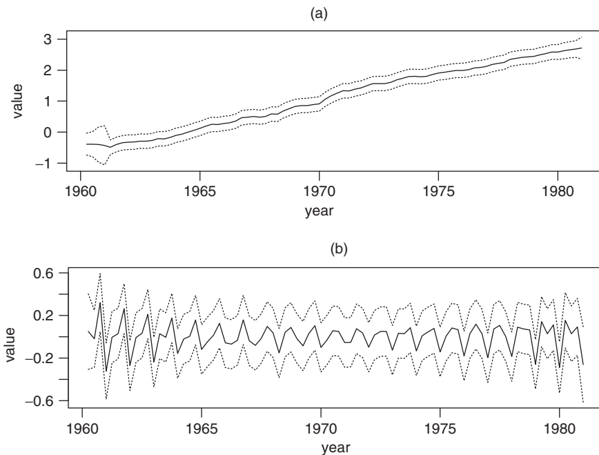
Figure 11.6. Smoothed components of fitting model (11.85) to the logarithm of quarterly earnings per share of Johnson and Johnson Company from 1960 to 1980: (a) trend component and (b) seasonal component. Dotted lines indicate pointwise 95% confidence regions.
