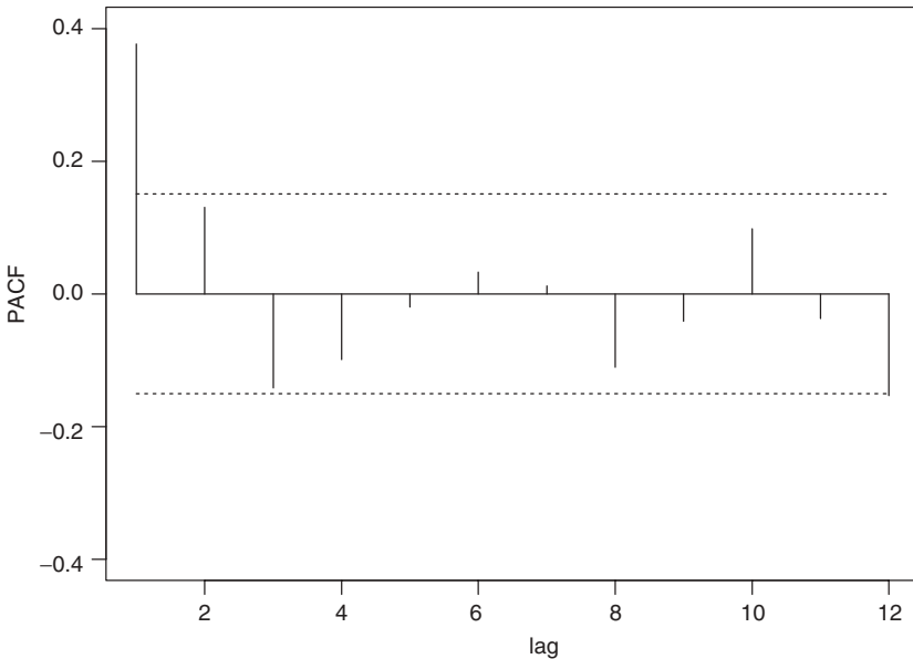
Figure 2.6. Sample partial autocorrelation function of the U.S. quarterly real GNP growth rate from 1947:II to 1991:I. The dotted lines give an approximate pointwise 95% confidence interval.
