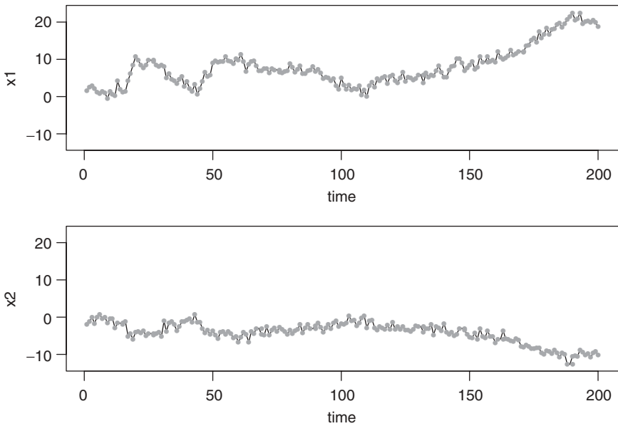
Figure 8.10. Time plots of a simulated series based on model (8.31) with identity covariance matrix for the shocks.
