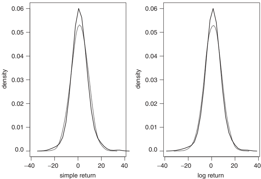
Figure 1.4. Comparison of empirical and normal densities for the monthly simple and log returns of IBM stock. The sample period is from January 1926 to December 2003. The left plot is for simple returns and the right plot for log returns. The normal density, shown by the dashed line, uses the sample mean and standard deviation given in Table 1.2.
