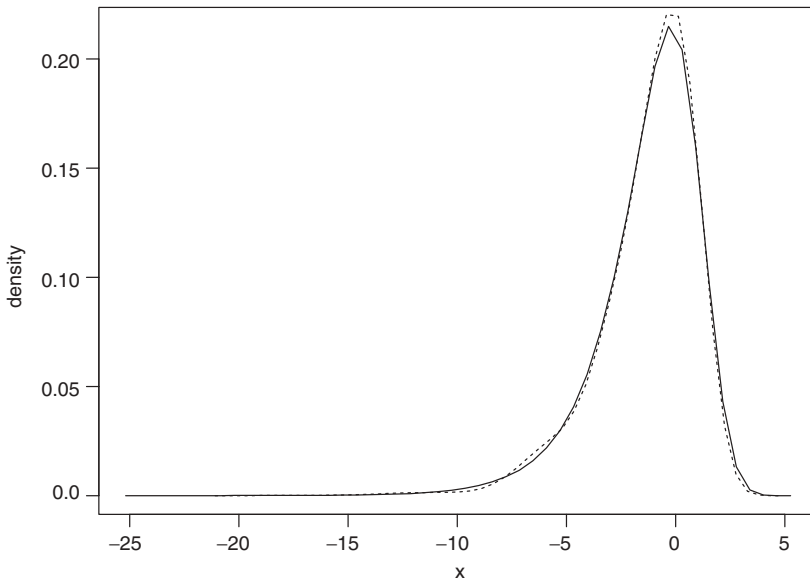
Figure 12.11. Density functions of \log(\chi_1^2) , solid line, and that of a mixture of seven normal distributions, dashed line. Results are based on 100,000 observations.
