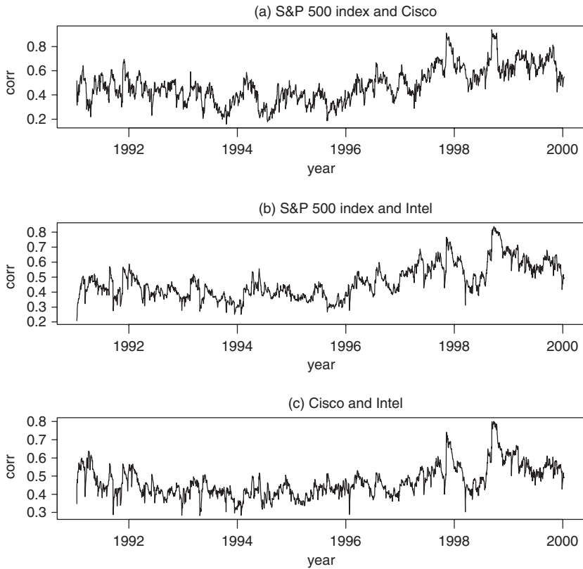
Figure 10.14. Time plots of fitted time-varying correlation coefficients between daily log returns of the S&P 500 index and stocks of Cisco Systems and Intel Corporation from January 2, 1991 to December 31, 1999.
