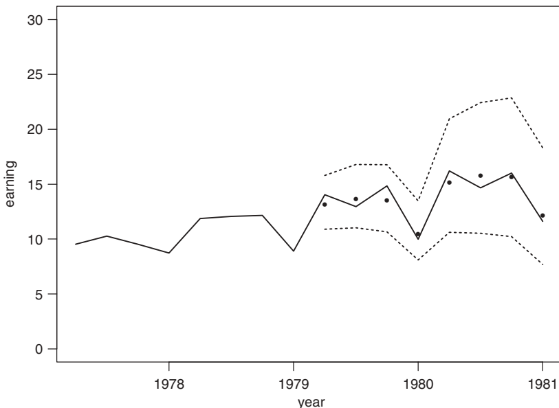
Figure 2.15. Out-of-sample point and interval forecasts for the quarterly earning of Johnson and Johnson. The forecast origin is the fourth quarter of 1978. In the plot, the solid line shows the actual observations, dots represent point forecasts, and dashed lines show 95% interval forecasts.
