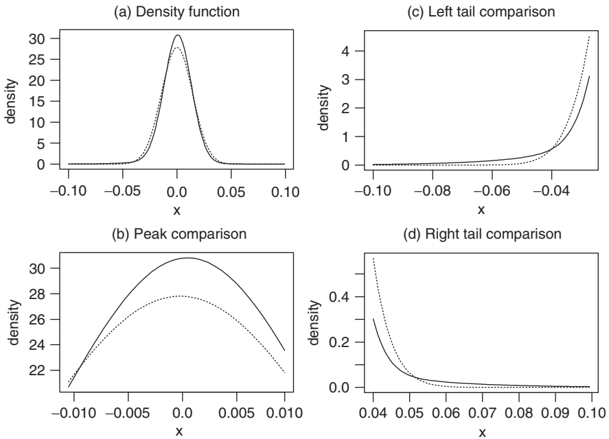
Figure 6.9. Density comparisons between a normal distribution and the distribution of Eq. (6.31). The dotted line denotes the normal distribution. Both distributions have mean zero and variance 2.0572 \times 10^{-4} . (a) Overall comparison, (b) comparison of the peaks, (c) left tails, and (d) right tails.
