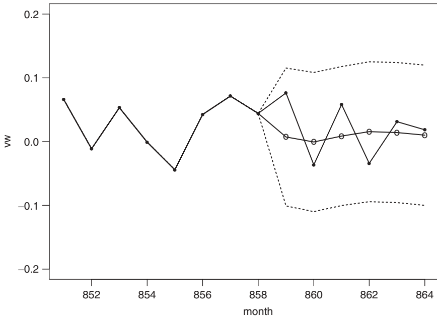
Figure 2.7. Plot of 1-step to 6-step ahead out-of-sample forecasts for the monthly log returns of the CRSP value-weighted index. The forecast origin is t = 858 . The forecasts are denoted by \circ and the actual observations by black dots. The two dashed lines denote two standard-error limits of the forecasts.
