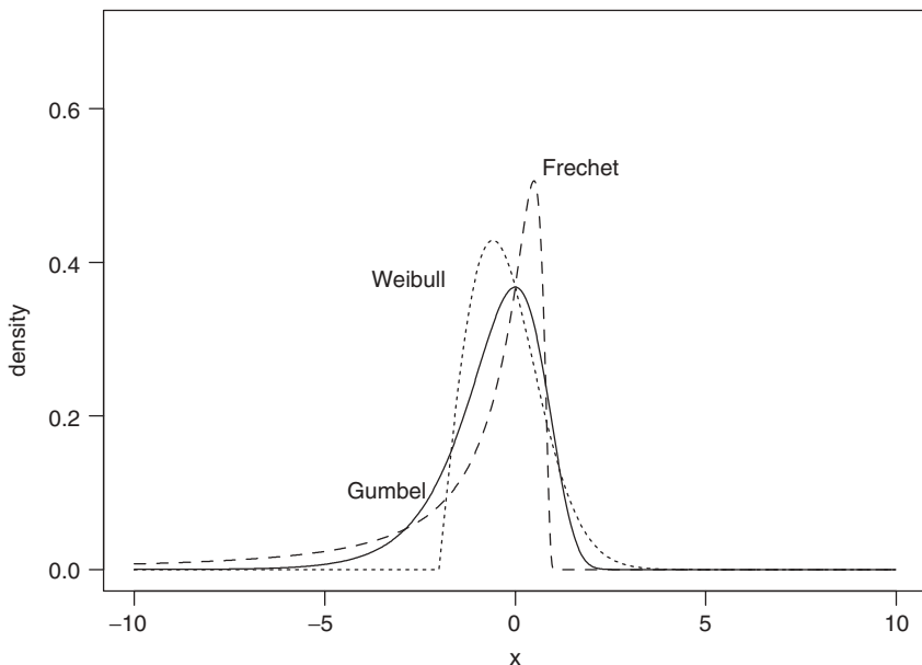
Figure 7.2. Probability density functions of extreme value distributions for minimum. The solid line is for a Gumbel distribution, the dotted line is for the Weibull distribution with k = 0.5 , and the dashed line is for the Fréchet distribution with k = -0.9 .
