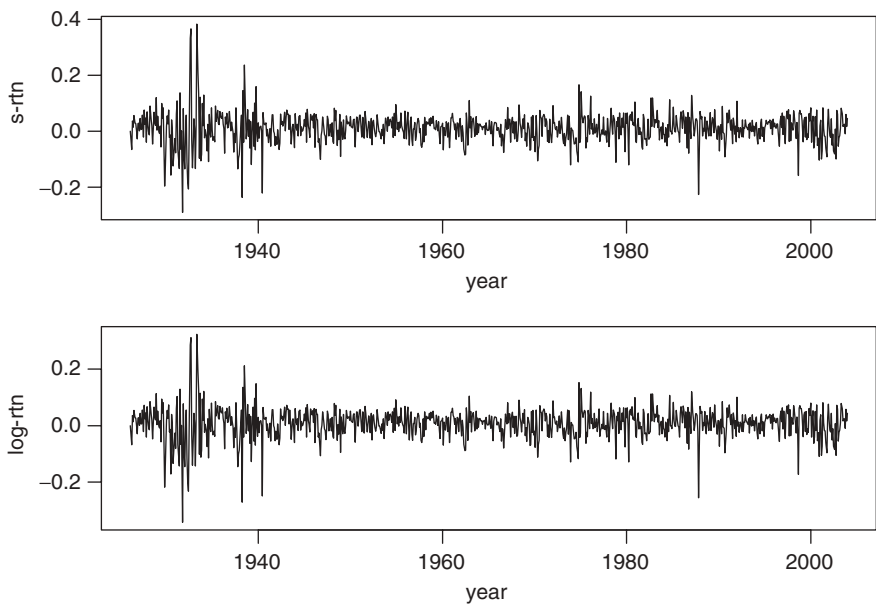
Figure 1.3. Time plots of monthly returns of the value-weighted index from January 1926 to December 2003. The upper panel is for simple returns, and the lower panel is for log returns.
