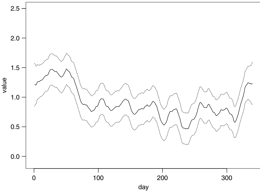
Figure 11.4. Smoothed state variable \mu_{r|T} and its 95% pointwise confidence interval for the daily log realized volatility of Alcoa stock returns based on the fitted local trend state-space model.
