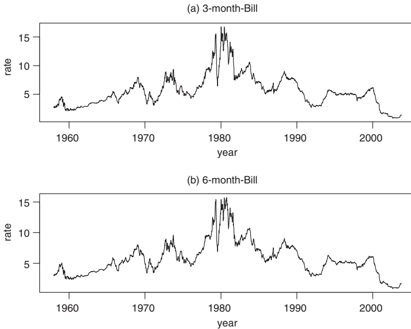
Figure 8.12. Time plots of weekly U.S. interest rate from December 12, 1958 to August 6, 2004. (a) The 3-month Treasury bill rate and (b) the 6-month Treasury bill rate. The rates are from the secondary market.
